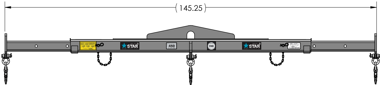
12' POSITION
