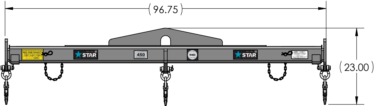
8' POSITION
