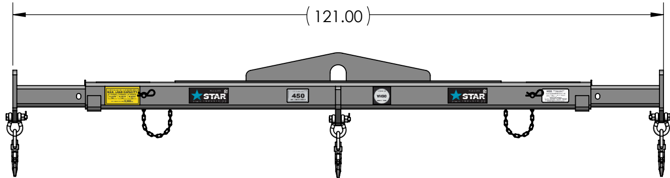
10' POSITION
