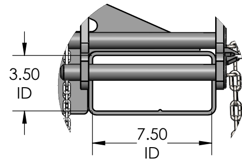
DETAIL A SCALE 1 : 6
