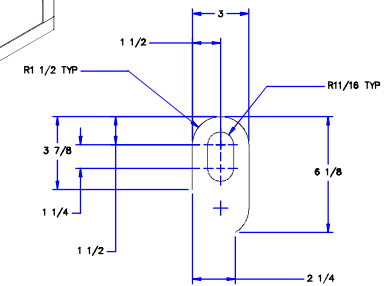
LIFTING EAR 5/8" PLATE PART # 1455-008 4 REQUIRED
