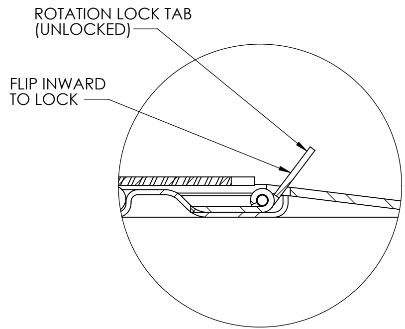
DETAIL B SCALE 1 : 2 DIMENSION TOLERANCE ± 1/4"
