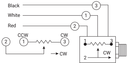
Potentiometer Model Wiring Diagram
