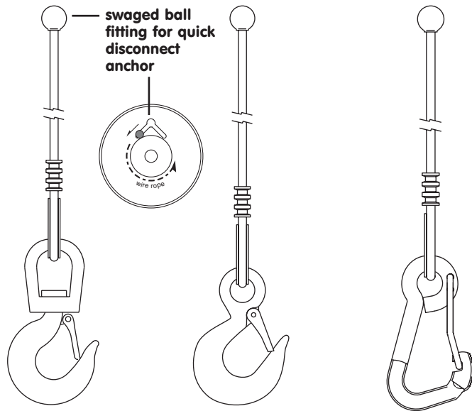
Swivel Hook
